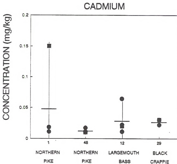
Figure 13. Comparison of replicate analyses from the same fish fillet. Squares represent the value of the initial determination while the circles represent cadmium from randomly selected tissue samples. Mean concentration (horizontal bar) and 95% confidence intervals are shown for the four samples.
